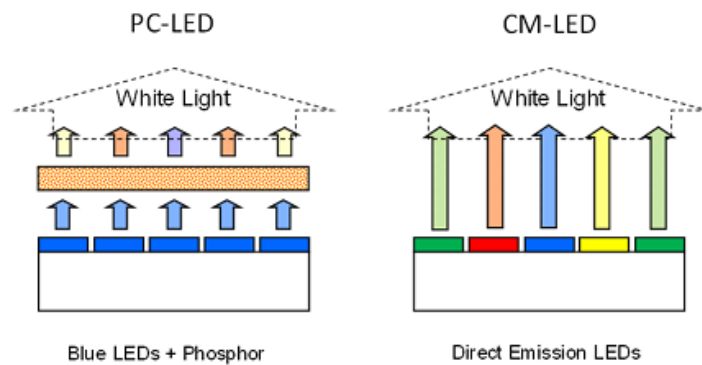
Figure 4.1: Schematics of the two main white LED architectures, Source: [14]
