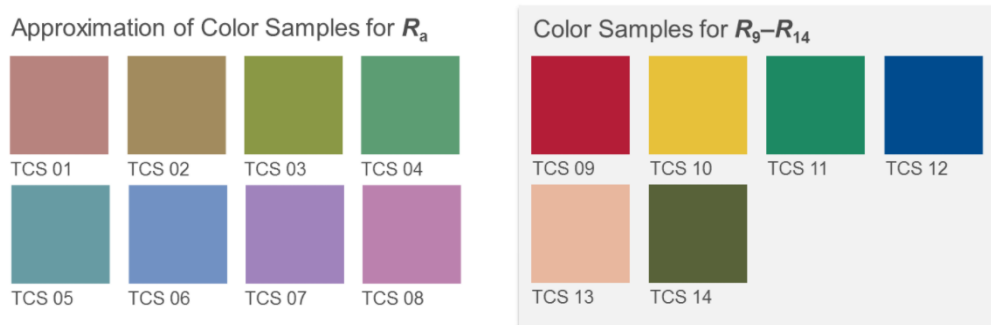
Figure 4.17: CIE 13.3-1995: Method of measuring and specifying colour rendering properties of light sources (CRI, R_a )
