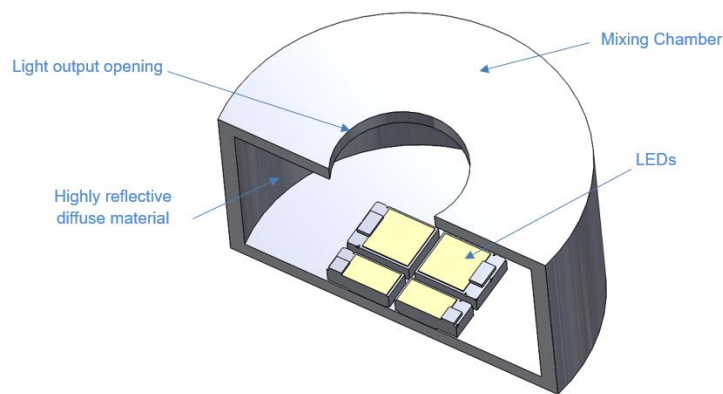
Figure 4.9: Colour Mixing: Mixing chamber and mixing light guide
