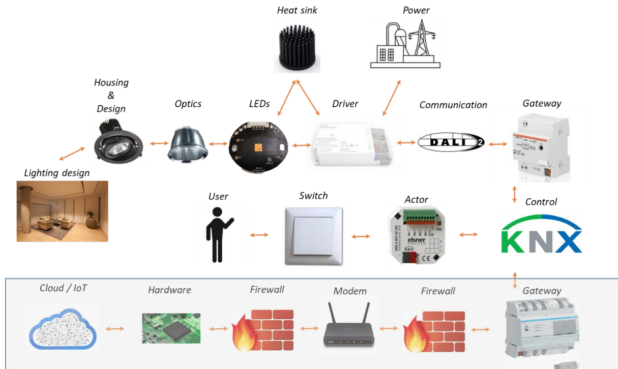
Figure 4.21: Components of an artificial lighting control system
