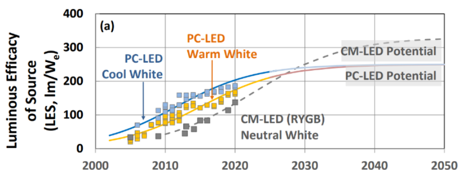
Figure 4.3: Historical and targeted efficacy levels of LEDs, Source: [14]
