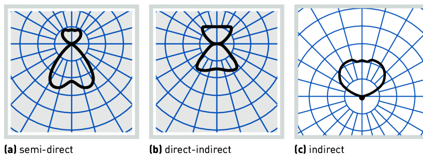
Figure 4.14: Exemplary luminous intensity distribution curves with indirect portion / trilux.com
