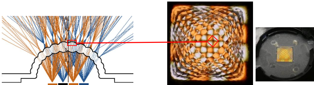
Figure 4.10: Colour Mixing: Mixing dome
