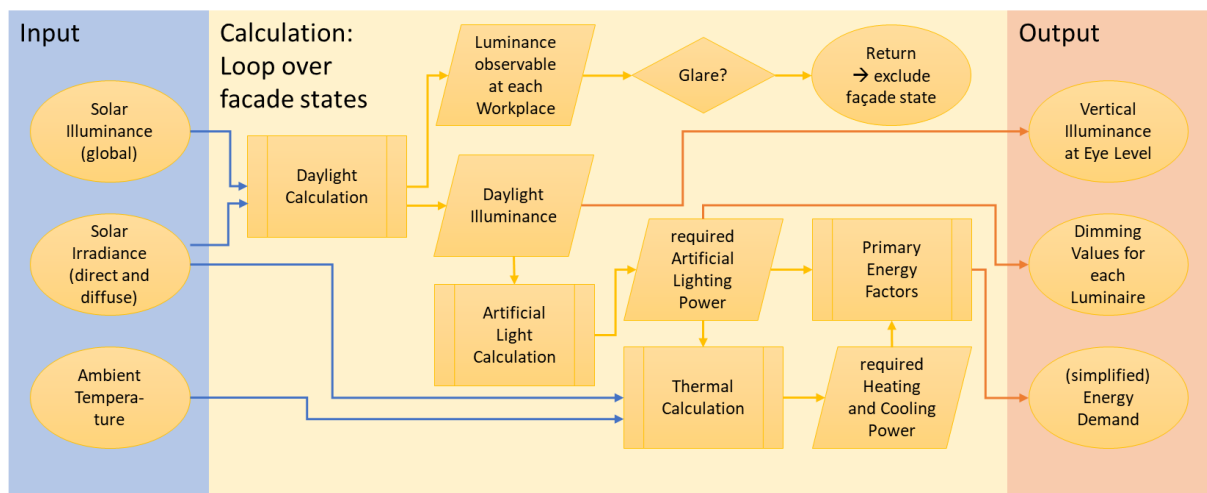
Figure 4.23: Control logic of the IndiLight-module
