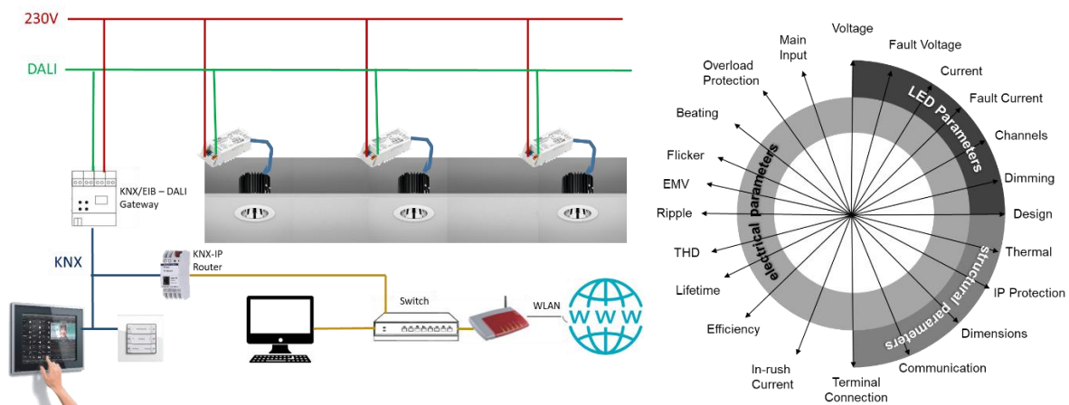
Figure 4.22: Exemplary integration scheme of DALI into a building management system (left) and different aspects to be considered in lighting controls (right)
