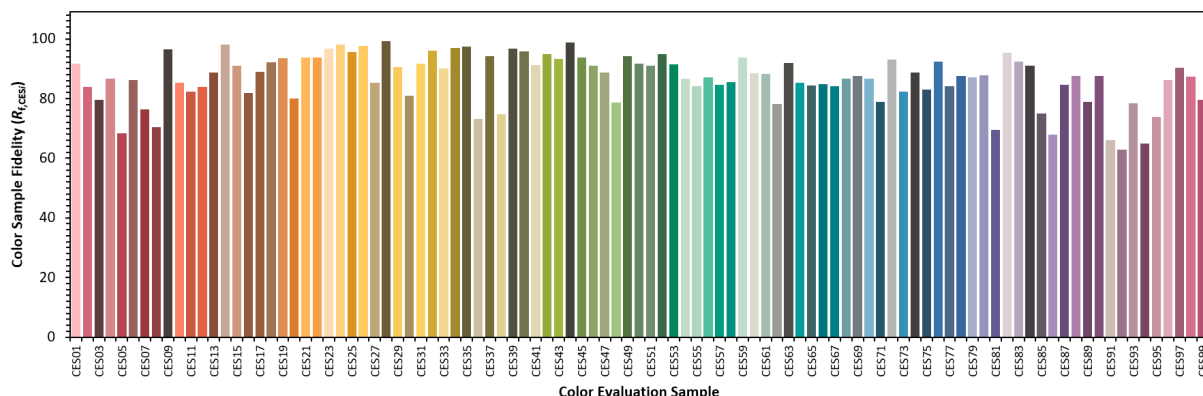
Figure 4.18: Fidelity Index R_f (TM-30) based on Colour Sample Fidelity for 99 colour samples: Example LED 4000 K, R_f = 87
