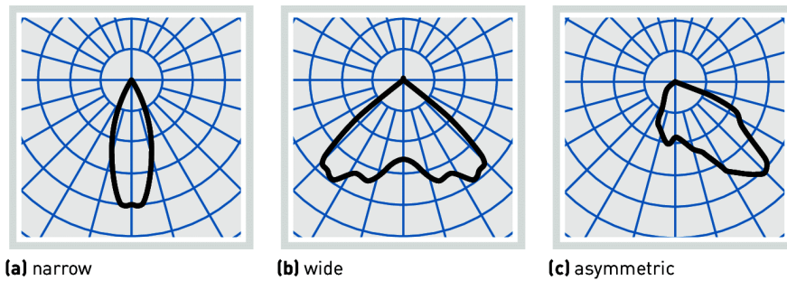
Figure 4.12: Exemplary luminous intensity distribution curves of direct-distribution luminaires / trilux.com
