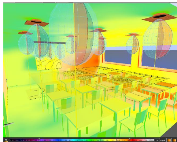
false-colour view of illuminances in a classroom
