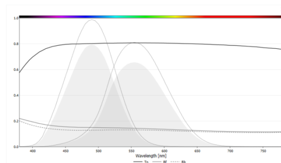
spectral properties for the glazing
