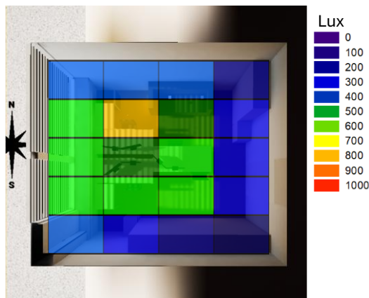
Horizontal illuminance values (daylight + electric light)
