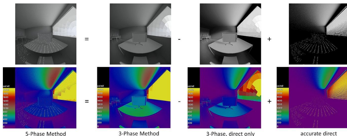
Example simulation showing the single steps of the 5-Phase Method: 5-Phase Method result, 3-Phase Method result, direct solar contribution from 3-Phase Method, and high accurate direct solar contribution (from left to right).
