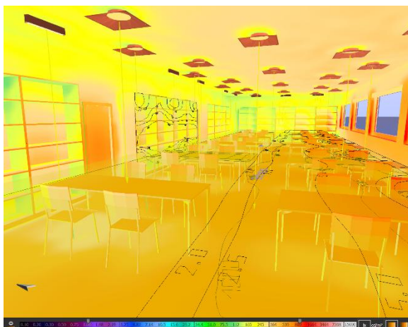
false-colour view of illuminances in the library (view 1)
