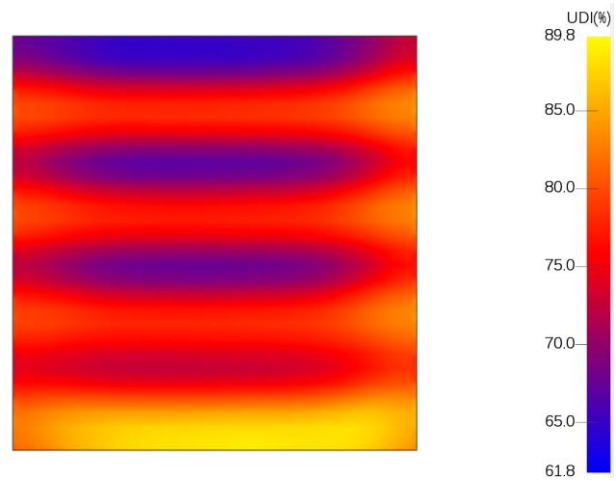
Fig. 2. Spatial distribution of UDI 100-3000 (%) for the hall in context (skylights)
