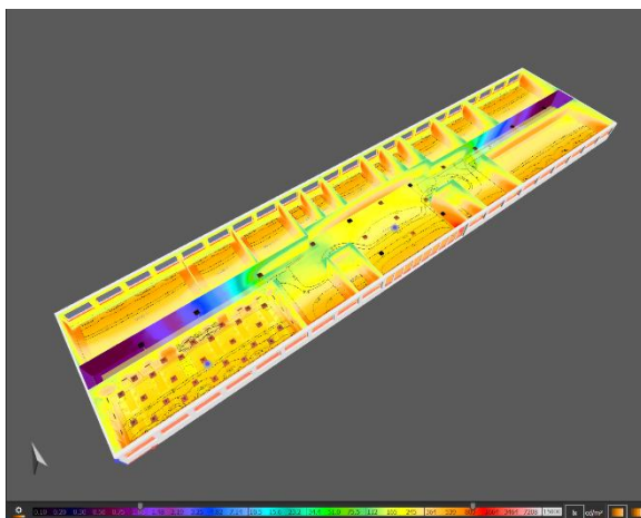
axonometric view of the whole floor, electric light only
