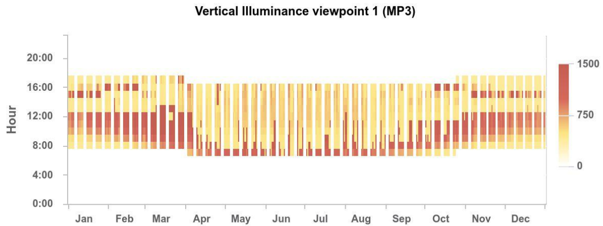
Figure 3: Annual vertical illuminance distribution at viewpoint in the office case
