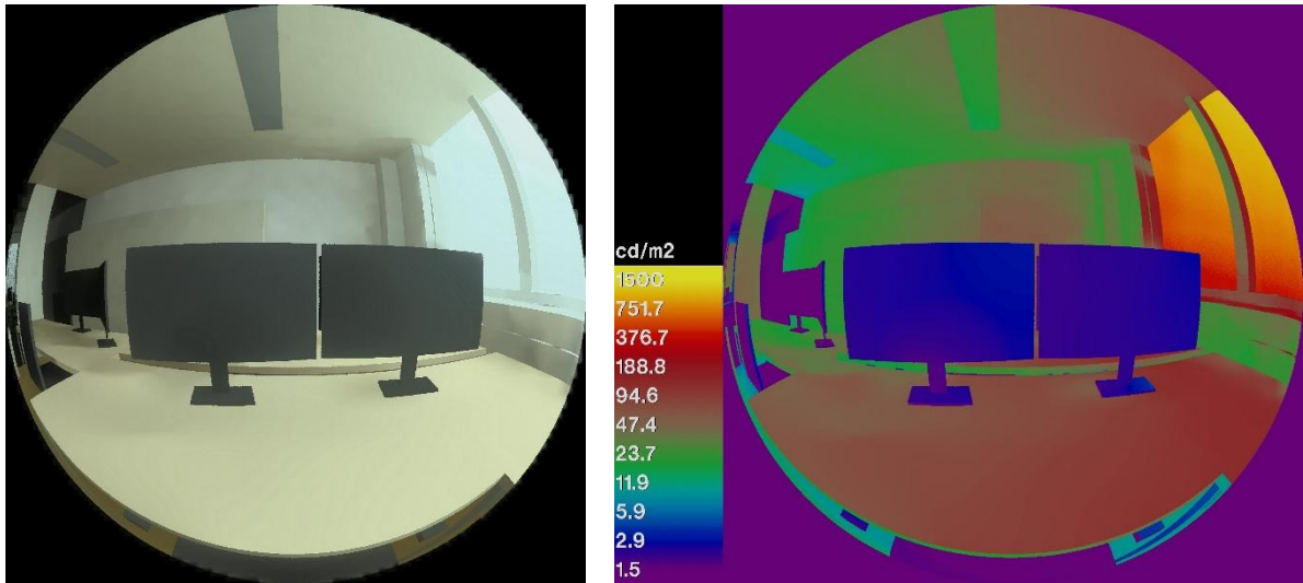
Hyperspectral rendering with Radiance for the reference office room under overcast sky conditions.
