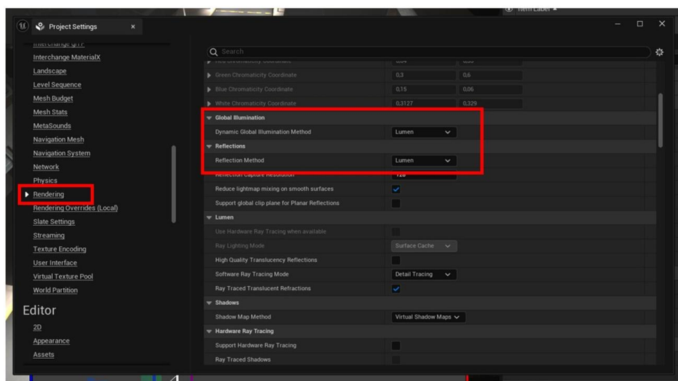
Figure 13: Lumen system for Global illumination and Reflection.
