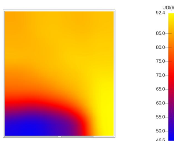
Fig. 1. Spatial distribution of UDI_{100-3000} (%) for the office in context (window is on the below, West)
