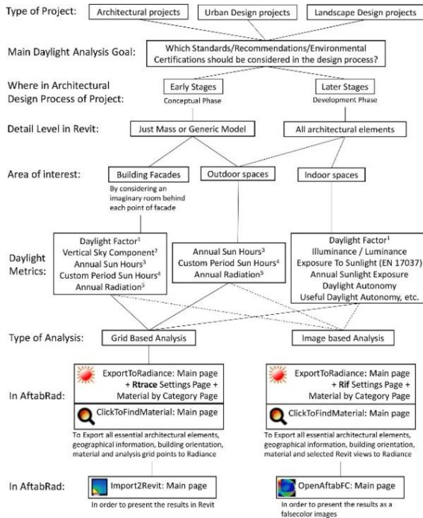
Figure 3: Flowchart (source: https://www.aftabsoft.net/AftabRad/images/flowchart.jpg )
