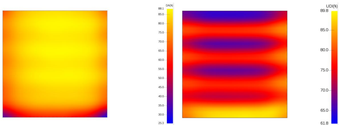
Figure 3: Spatial distribution of DA [%] (left) and UDI 100-3000 [%] (right) for the hall in context (Location: Beijing)
