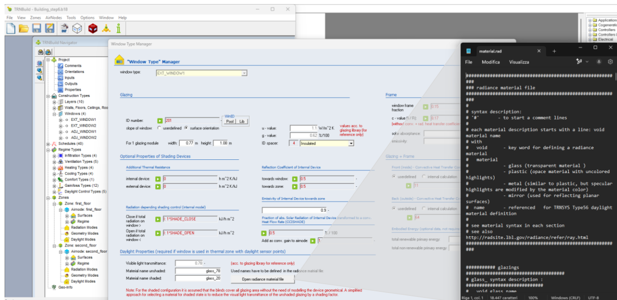
Figure 8: Radiance material files - "Window Type Manager".
