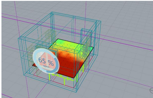
average illuminance spatial distribution
