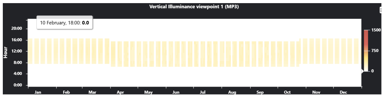
Fig. 4. Hourly vertical illuminance in lux at viewpoint from day- and artificial light
