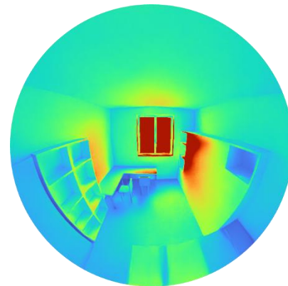
Falsecolour render view completed December 21, 12.30
