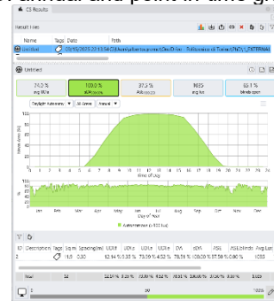
sDA annual and point-in-time graphs
