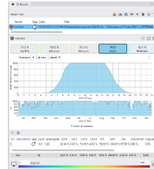
average illuminance annual and point-in-time graphs
