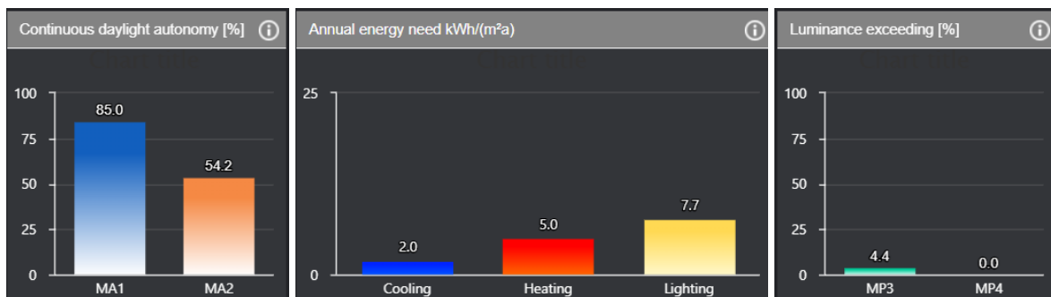
Figure 2: Daylight autonomy, annual energy need, and luminance exceeding in the office case
