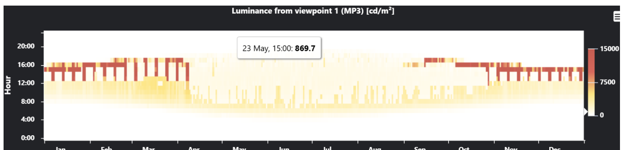
Fig. 1. Hourly maximum luminance in \text{cd/m}^2 at the façade seen from viewpoint
