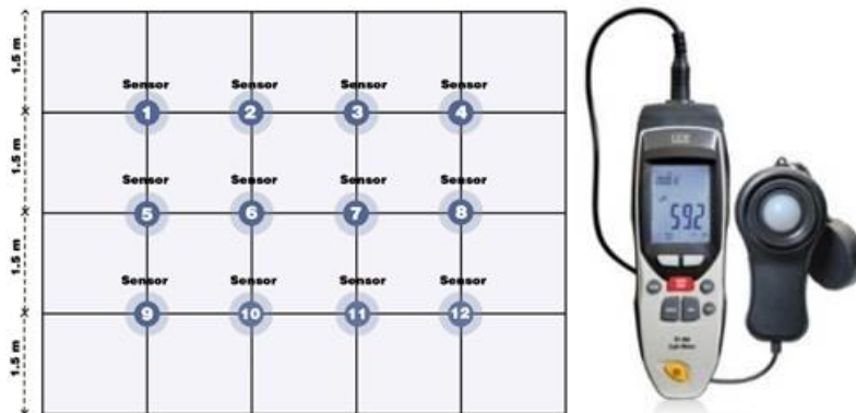
Figure 1. Sensor grid layout and measurement setup for daylight simulation validation.
