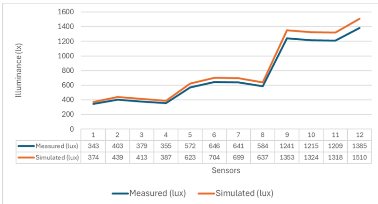
Figure 2. Comparison of measured and simulated illuminance values at sensor points.
