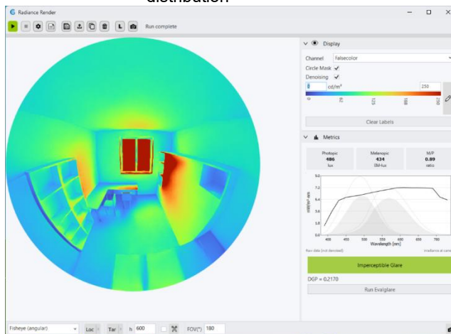
Spectral Radiance rendering window
