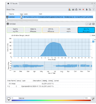
blinds annual usage profile for daylight availability workflow
