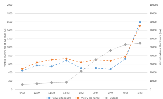
Vertical daylight illuminance values
