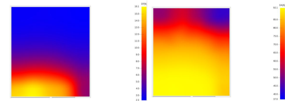
Figure 6: Spatial distribution of DF [%] (left) and DA [%] (right) for the office in context (Location: Beijing)
