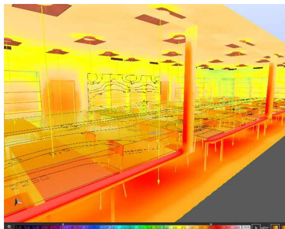
false-colour view of illuminances in the library (view 2)
