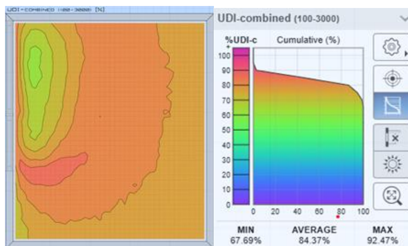
Figure 3: Useful Daylight Illuminance (100-3000 lx) simulation results for an office room using Andrew Marsh, Dynamic Daylight ( https://drajmarsh.bitbucket.io/daylight-box.html )
