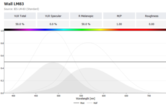
spectral properties for the material
