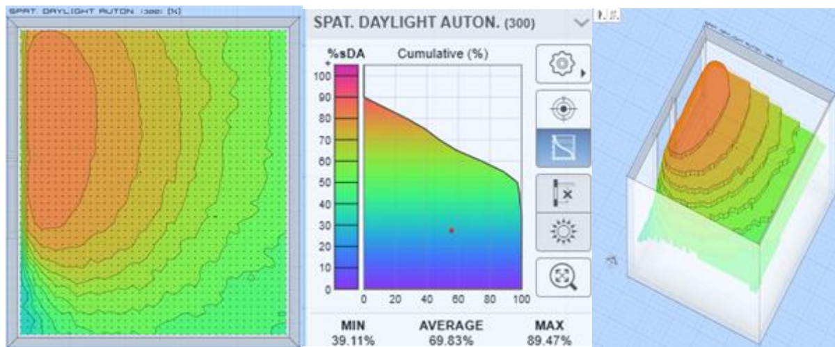
Figure 3: Spatial Daylight Autonomy 300/50 simulation for an office room using Andrew Marsh, Dynamic Daylight ( https://drajmarsh.bitbucket.io/daylight-box.html )
