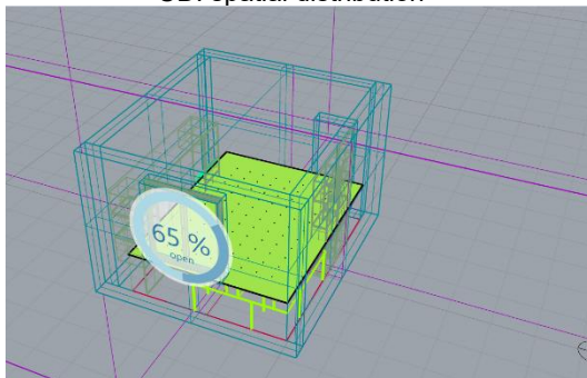
sDA spatial distribution
